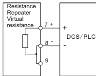
3-wire (+, +, -)
