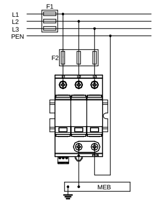
Three-phase TN-C system
