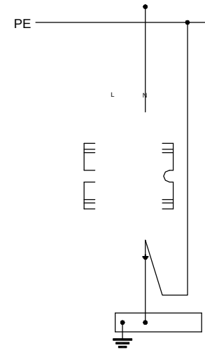
Single phase TN system
