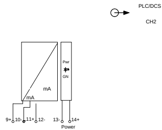
24V DC, single input, double current / voltage output
